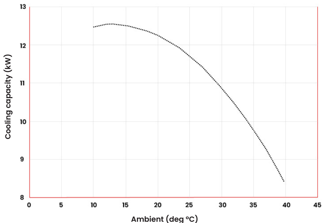
Cooling capacity vs Ambient @ 25°C coolant
